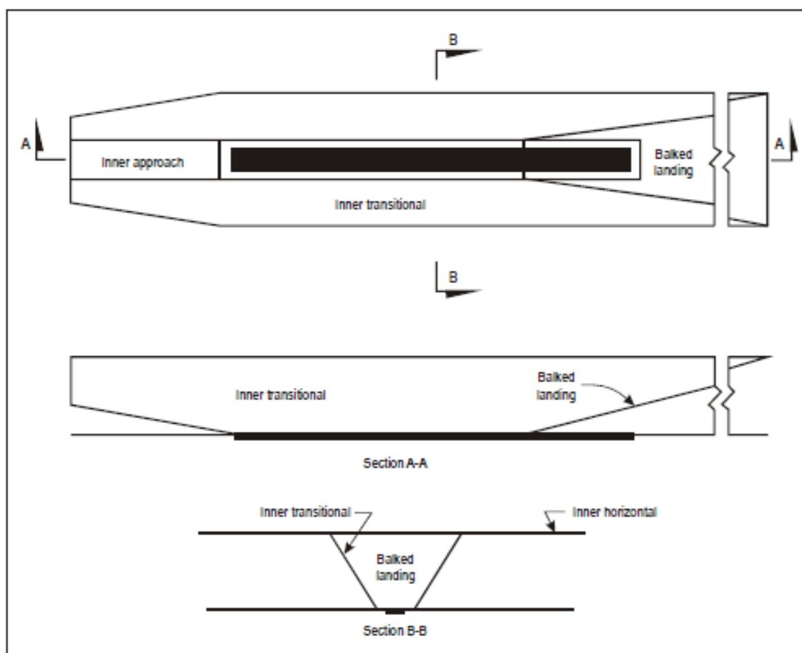
Figure 6. Inner approach, inner transitional and balked landing obstacle limitation surfaces (Figure 4-3 ICAO Annex 14)
