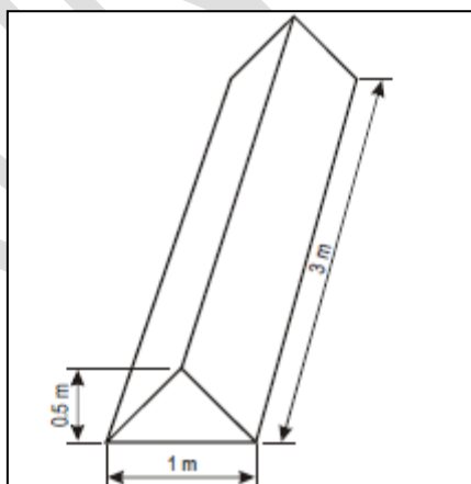
Figure 40. Boundary Markers (Figure 5-34 ICAO Annex 14)
