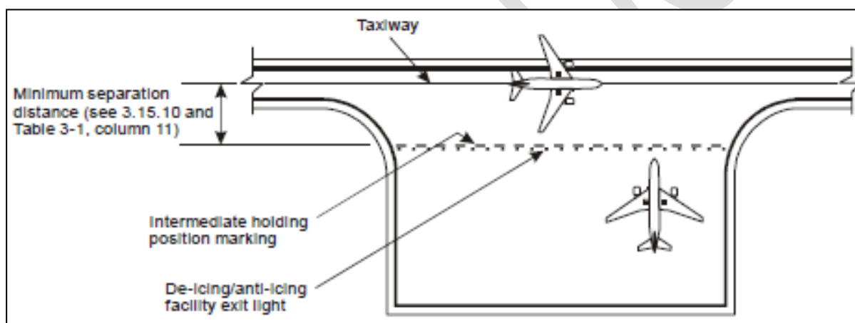
Figure 34. Typical remote de-icing/anti-icing facility (5-28 ICAO Annex 14)
