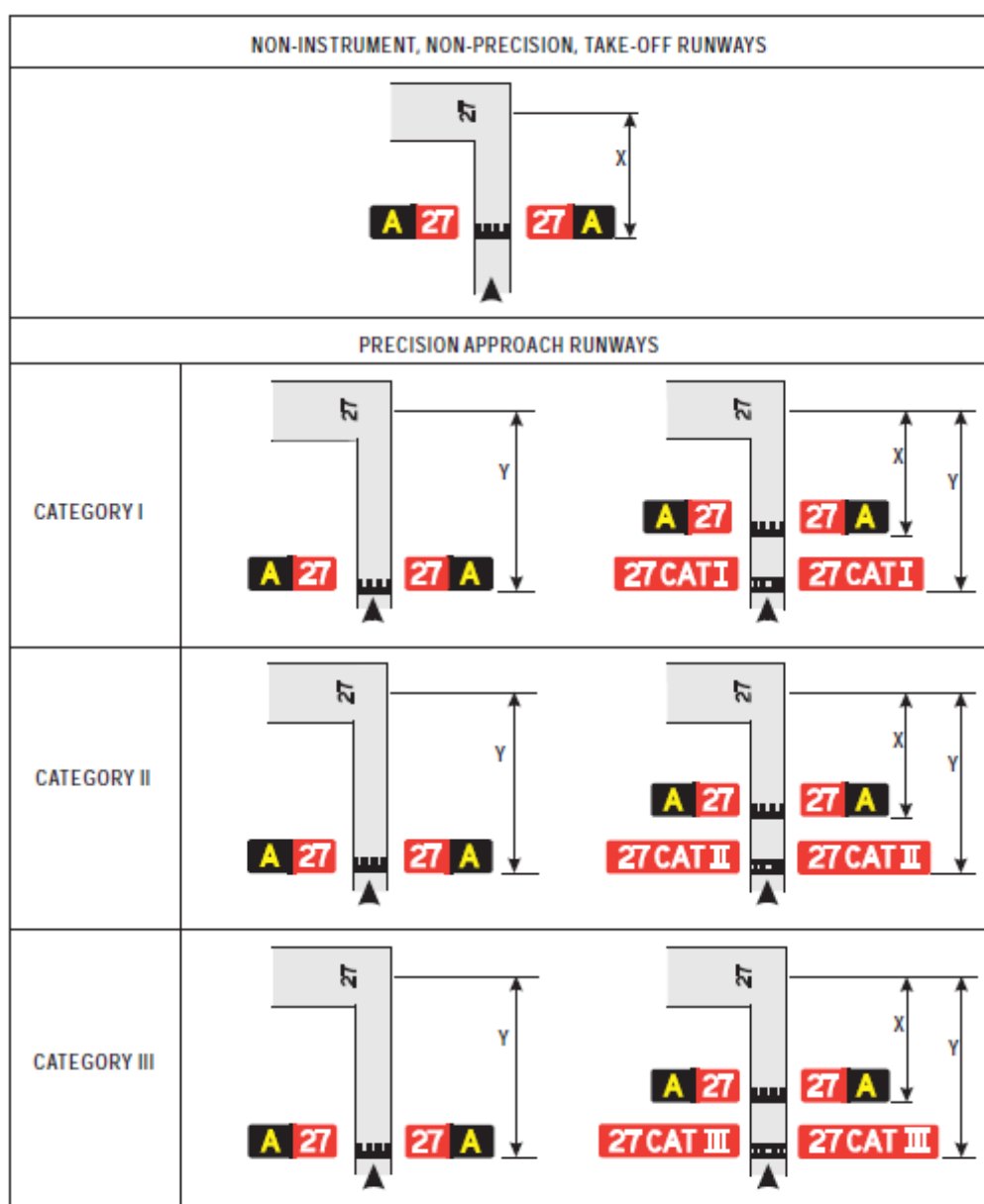
Figure 38. Examples of sign position at taxiway/runway intersections (Figure 5-32 ICAO Annex 14)
