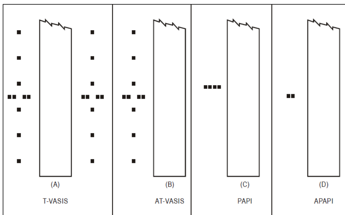
Figure 22. Visual approach slope indicator system (Figure 5-16 ICAO Annex 14)
