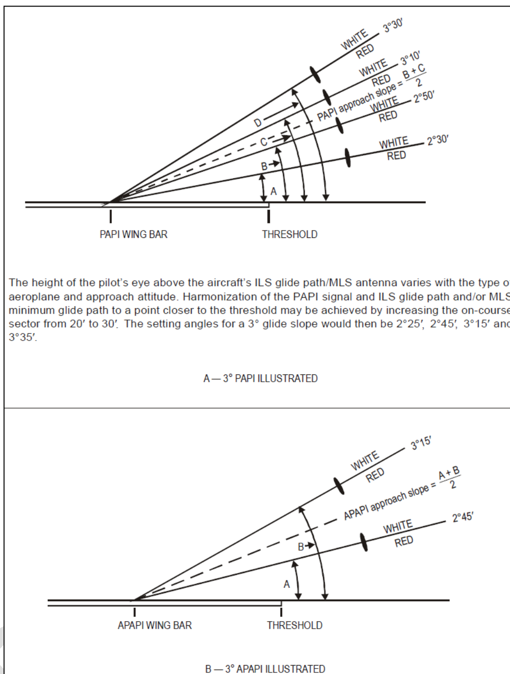
Figure 26. Light beams and angle of elevation setting of PAPI and APAPI (Figure 5-20 ICAO Annex 14).
