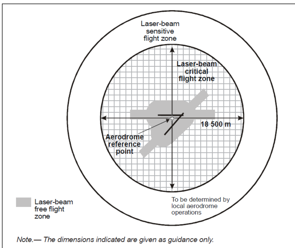
Figure 17. Protected Flight Zones (Figure 5-11 ICAO Annex 14)
