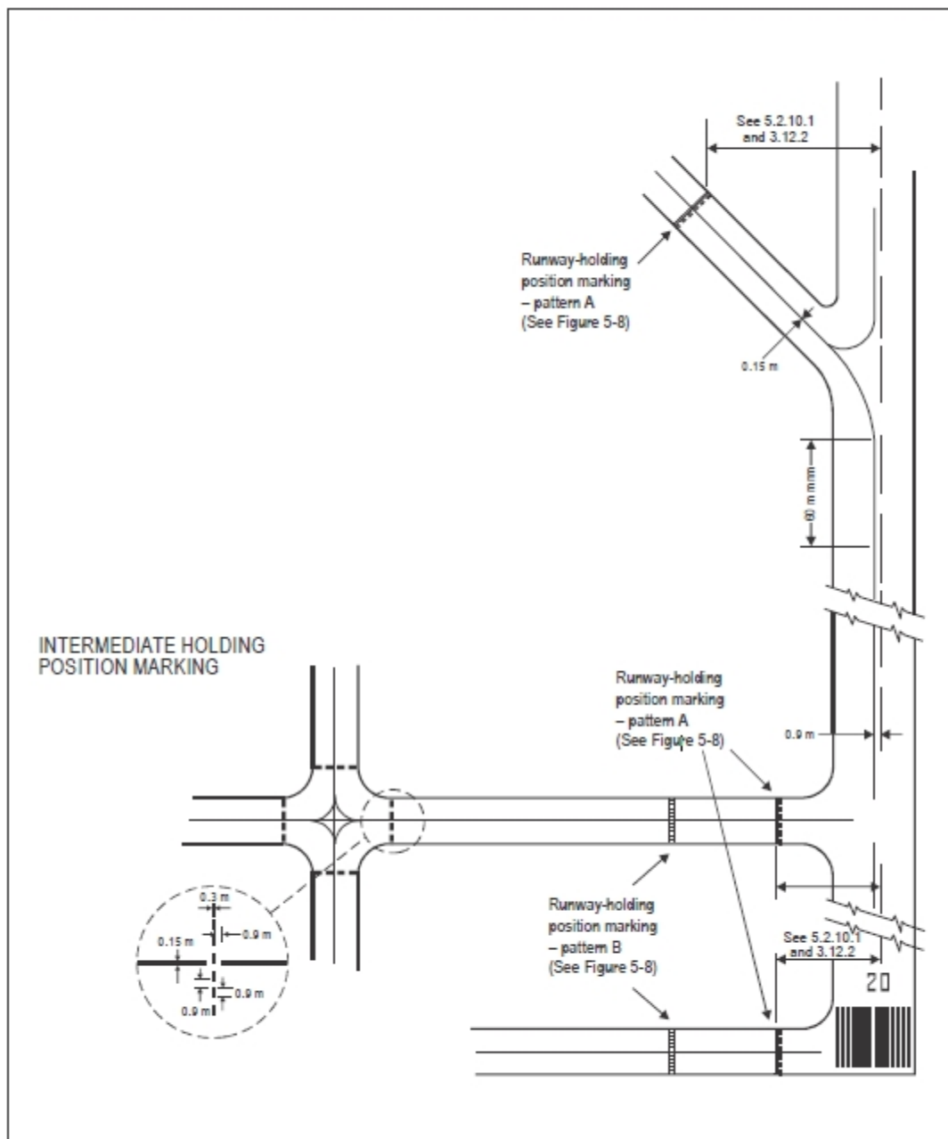
Figure 12. Taxiway markings (shown with basic runway markings) (Figure 5-6 ICAO Annex 14)
