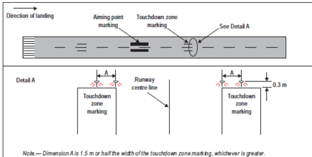
Figure 30. Single touchdown zone lighting (5-24 ICAO Annex 14)
