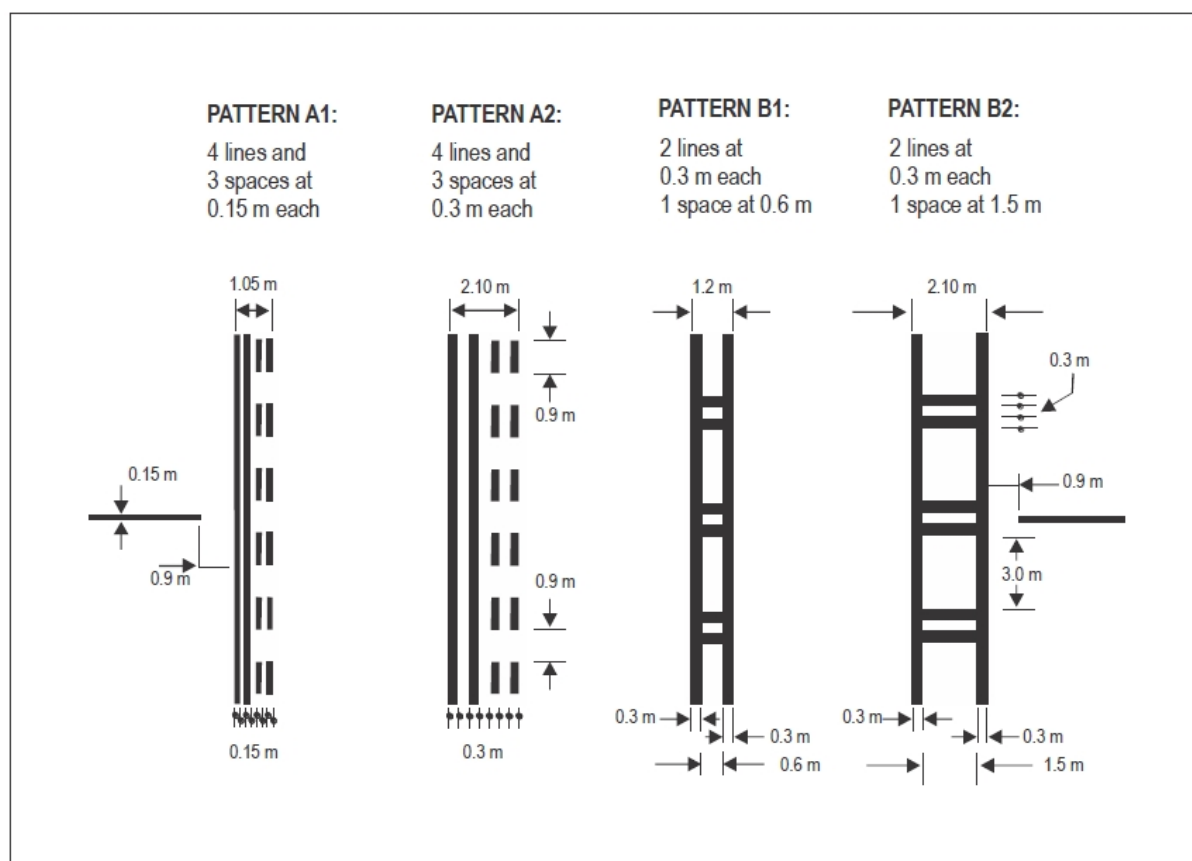
Figure 14. Runway holding position markings (Figure 5-8 ICAO Annex 14).
